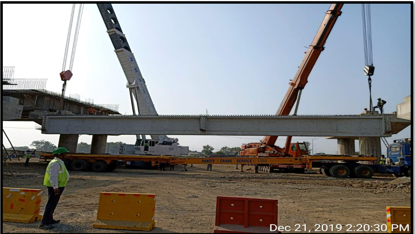
Girder Erection at VUP Ch 15+725
