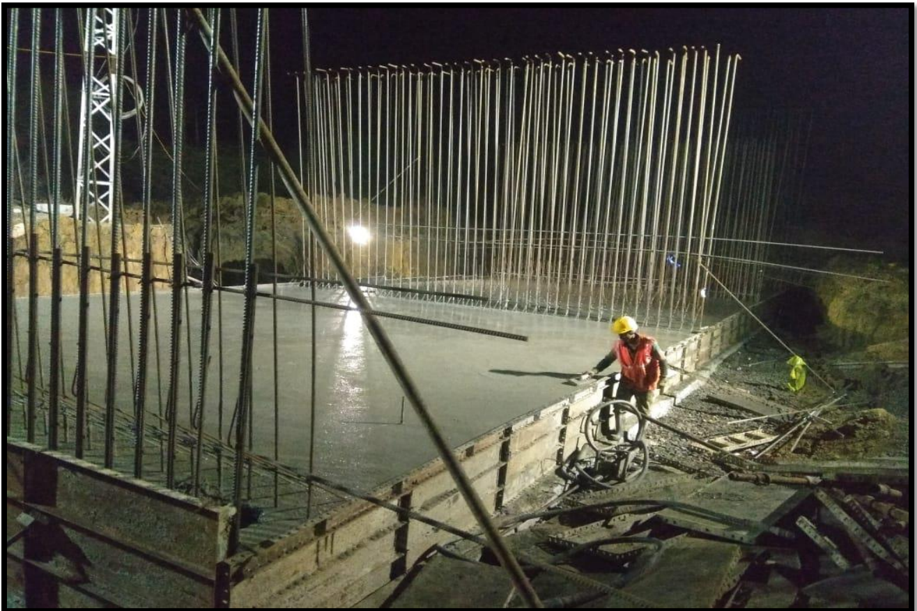
Raft of Minor Bridge at Ch. 12+380 (BHS)
