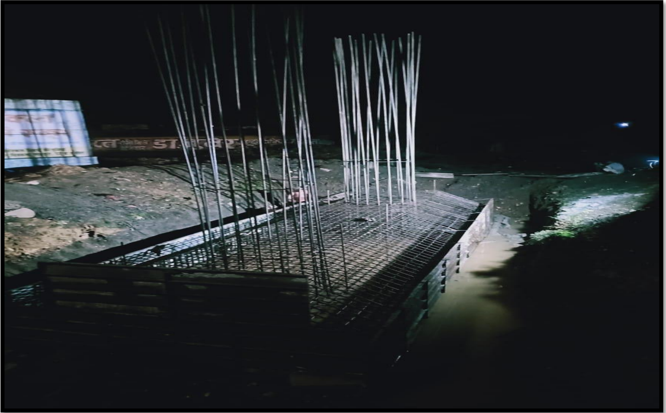
Steel & Reinforcement Work @ Ch.58+128 (Flyover)
